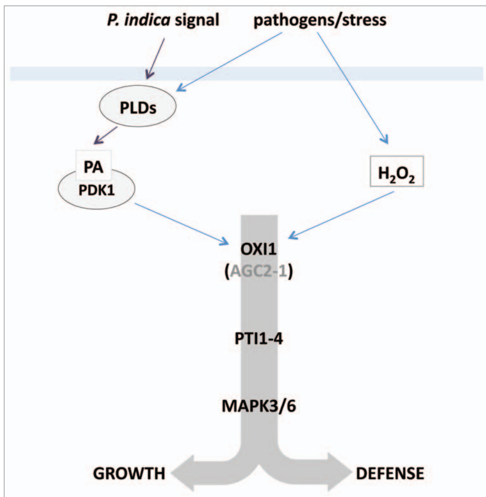
Figure 1. The beneficial fungus Piriformospora indica stimulates PA synthesis which activates PDK1 and subsequently OXI1 and AGC2-2. On the other hand, OXI1 can also be activated by environmental challenges, including pathogens in a PDK1-independent manner via H 2 O 2 . PTI1-4 and the MAPKs MPK3 and 6 are downstream factors of OXI1 and regulate the balance between growth and defense responses.
